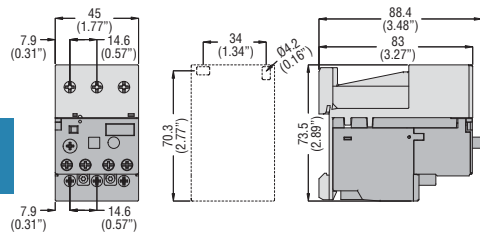
RF...200 thermal relay with links G372 and G373
